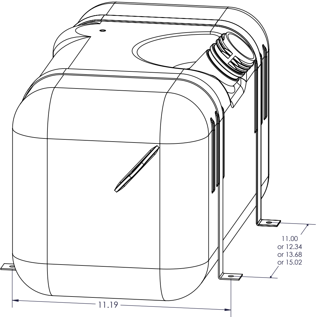
Recommended Mounting Hole Pattern
